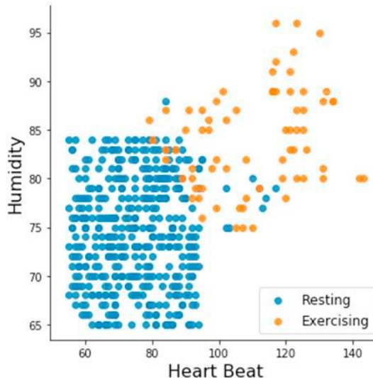
FIGURE 5(a): K-Means Clustering forming 2 clusters for Temperature Vs Heart Beat & Humidity Vs Heart Beat respectively
