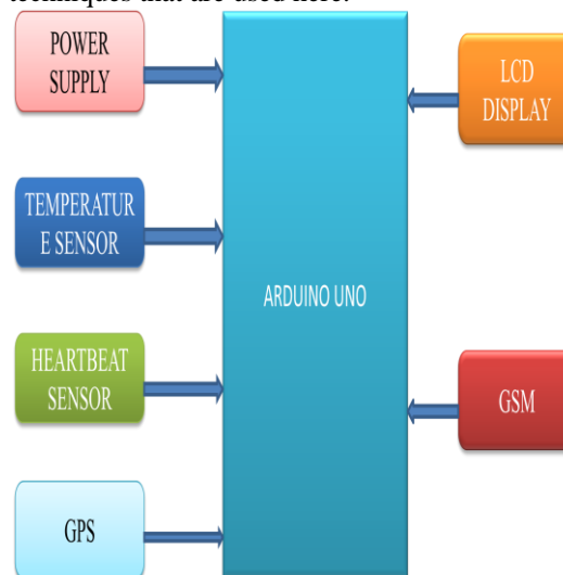
FIGURE 2: IOT Based Soldier health and Tracking System
