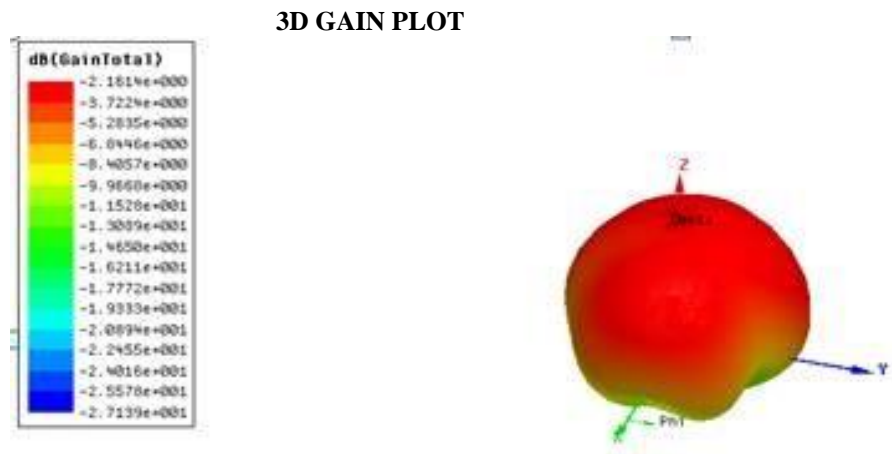
Fig.6. 3D gain plot
