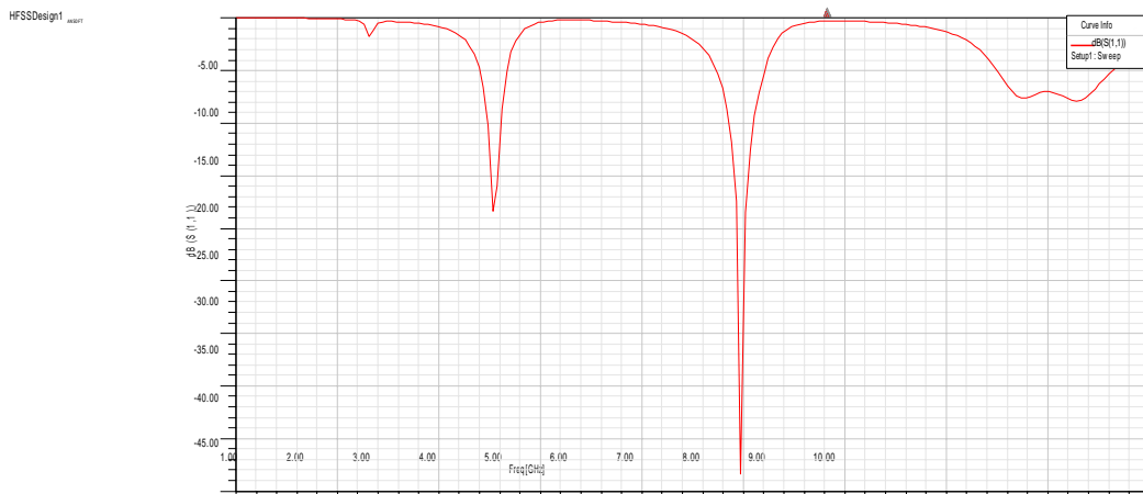
Fig. 2. Graph of Return loss versus Frequency.
