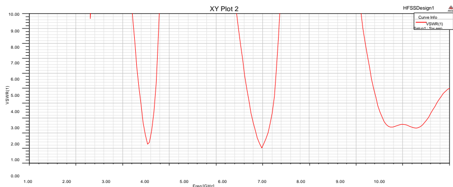
Fig. 3. Frequency versus VSWR.
