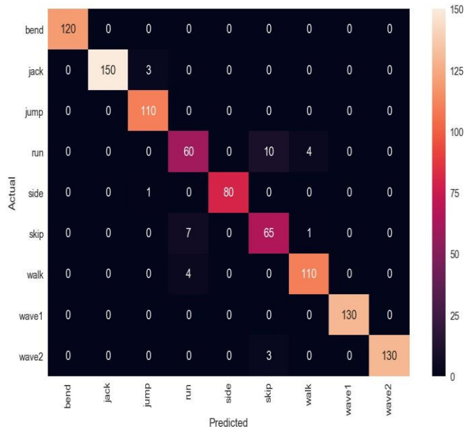
Fig. 2. Confusion Matrix for recognising 9 activities on Weizmann Dataset using VGG-16 Convolutional Neural Network
