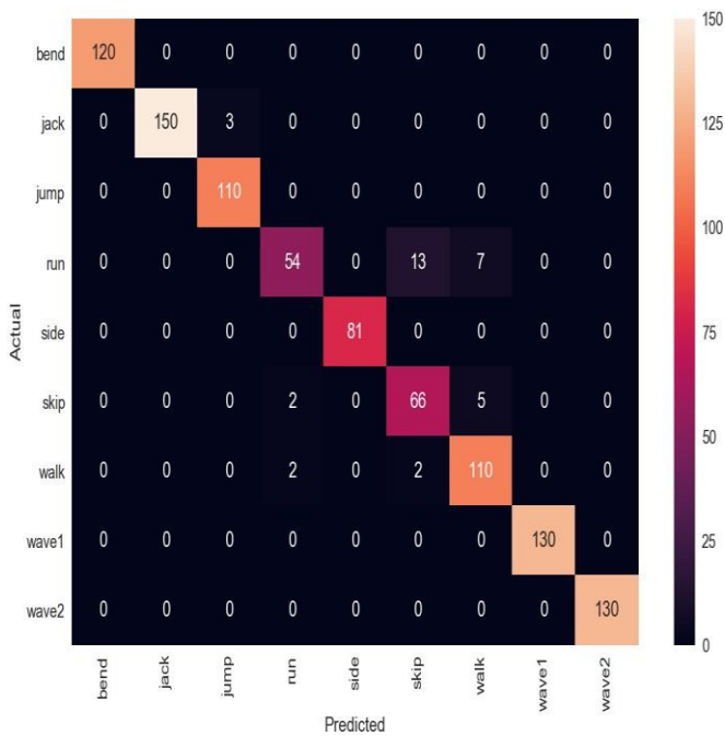
Fig. 3. Confusion Matrix for recognising 9 activities on Weizmann Dataset using VGG-19 Convolutional Neural Network
