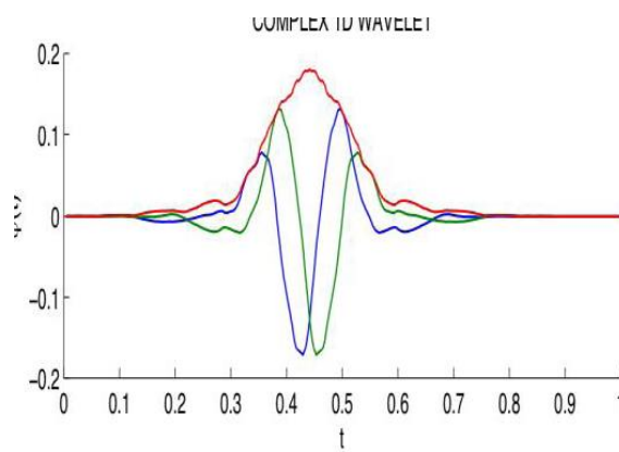
Fig 1: Complex wavelet
