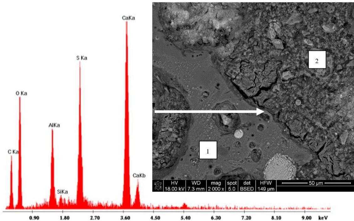
Figure 12. Microanalysis and image of fettringite in the interfacial transition zone (ITZ) of lightweight concrete with initially saturated aggregate (1S); 1—LWA and 2—cement paste.
