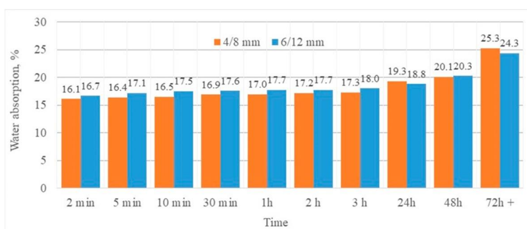
Figure 2. The development of water absorption of a sintered fly ash aggregate over time.
