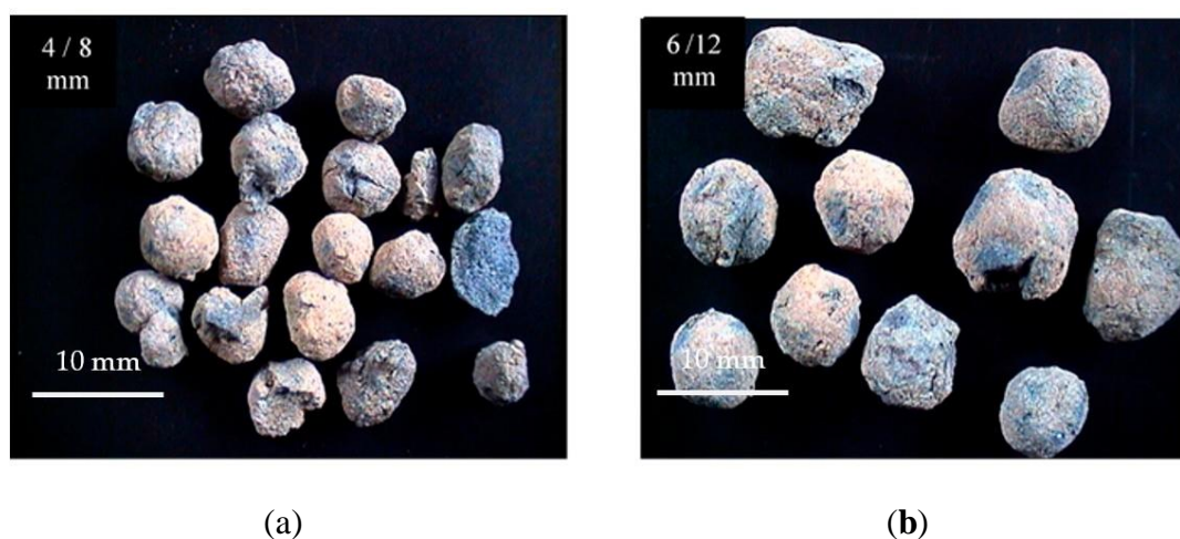
Figure 1. Sintered fly ash aggregate: (a) fraction 4/8 mm and (b) fraction 6/12 mm.
