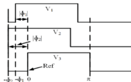
Fig. 4: Mode 2: Winding Voltages when -\phi_2 < -\phi_1 < 0
