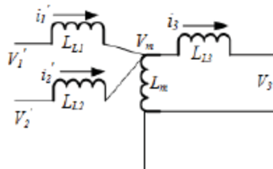
Fig. 2: Equivalent Circuit of Transformer for TAB Converter
