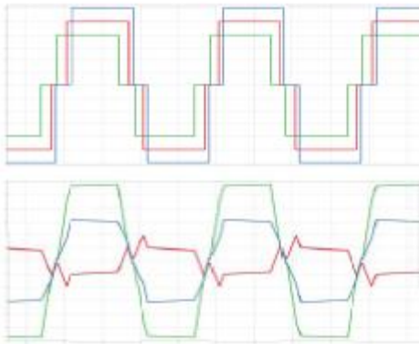
Fig. 7: Transformer Winding Voltages and Currents The winding voltage expressions using harmonic model for each port with quasi-square voltage waveforms are given in equations (29)-(31). The three winding currents are derived here using the winding voltage harmonics. The harmonic current vector expressions for any harmonic component 'n', using the voltage vectors, are shown in equations (32)-(34). The active power flow expressions for each port are derived over a switching cycle and are expressed in (35)-(37). The current expressions in vector form are derived in terms of different parameters, and are given in equations(38)-(40). The RMS current expressions are shown in equations (41)-(43).
