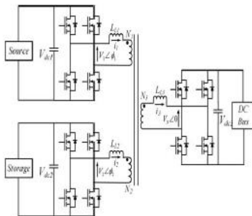
Fig. 1: Triple Active Bridge(TAB) Phase-Shifted DC-DC Converter
