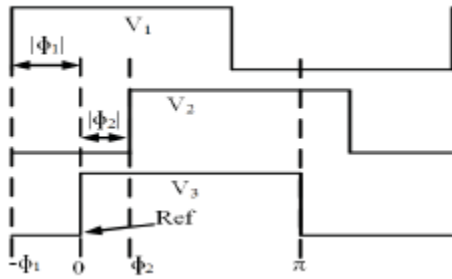
Fig. 5: Mode 3: Winding Voltages when -\phi_1 < 0 < \phi_2
